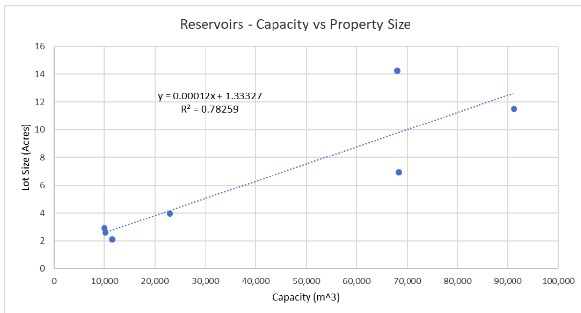
Figure 10 – Water Storage in Ground Reservoir Property Size Curve
