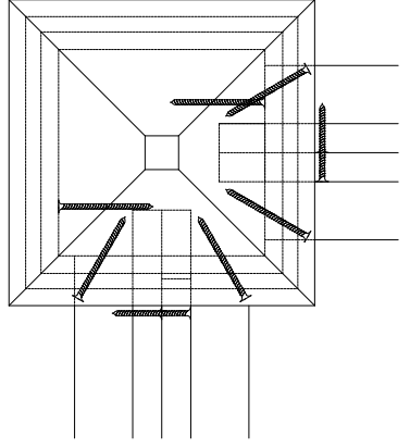
180° POST JOINT AND CAP DETAIL
